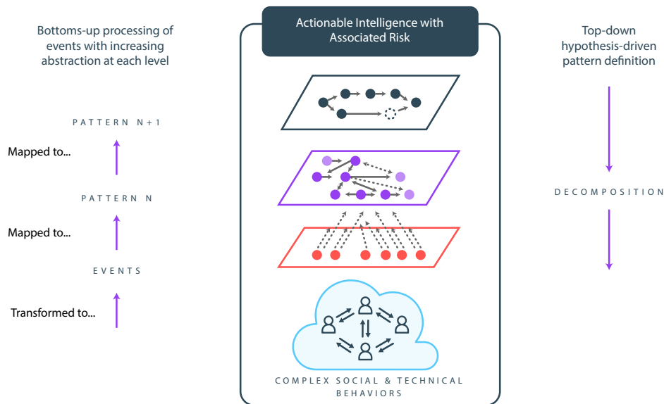
Figure 3. Hierarchical Complex Event Processing (HCEP)
